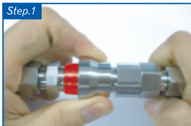
Pull the body sleeve toward the stem.
