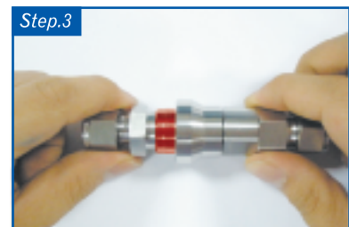
Connections is complited when it "clicks"
