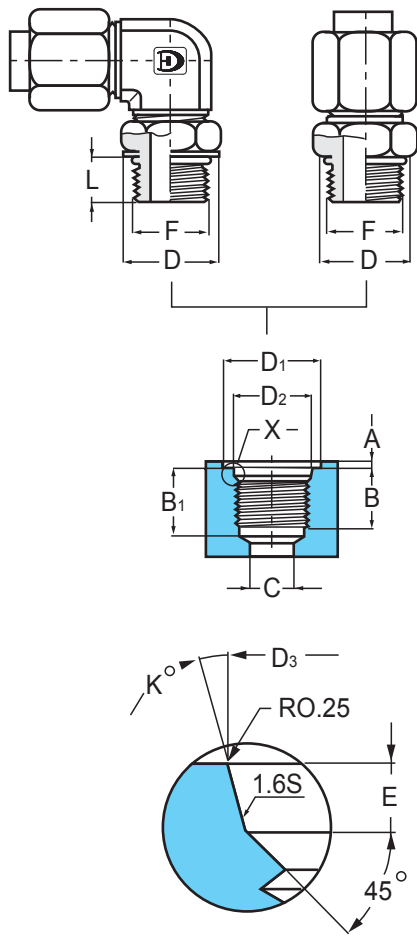
Detail X
